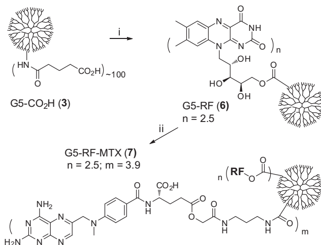
Scheme 2. Synthesis of PAMAM G5-RF n -MTX m nanoconjugate 7 . Reagents and conditions: (i) EDC, 4-dimethylaminopyridine (DMAP), riboflavin, DMF, rt, 24 h; (ii) 1 , EDC, DMAP, DMF, rt, 24 h.
