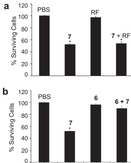
Figure 3. Cytotoxicity of G5-RF 2.5 -MTX 3.9 ( 7 , 30 nM) in KB cells tested under various control conditions. (a) Effect on cell growth of PBS (control), G5-RF 2.5 -MTX 3.9 ( 7 , 30 nM), RF (30 \mu M), and a mixture of 7 (30 nM) and RF (30 \mu M), (b) effect on cell growth of PBS, G5-RF 2.5 -MTX 3.9 ( 7 , 30 nM), G5-RF 2.5 ( 6 , 30 \mu M), and a mixture of 6 (30 \mu M) and 7 (30 nM). *The p value for each of the data set is <0.005 compared to PBS.
