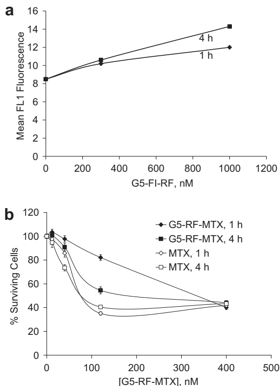
Figure 2. (a) Dose-dependent binding and uptake of G5-RF 6.3 -FI 1.3 5 in KB cells. The cells were incubated with different concentrations (300 and 1000 nM per conjugate basis) of RF dendrimer 5 for 1 or 4 h in HBSS buffer. The cells were then rinsed and resuspended in PBS buffer, and fluorescence intensity was measured in a flow cytometer; (b) dose-dependent cytotoxicity of G5-RF 2.5 -MTX 3.9 7 and free MTX in KB cells. Cells were treated with 7 for 1 or 4 h at four different concentrations (per MTX basis) in a RF-free HBSS-BSA medium, washed and followed by incubation in a conjugate-free growth medium for 3 days. The inhibition of cell growth induced was quantified by an XTT assay, which is based on the conversion of XTT to formazan by the active mitochondria of live cells.
