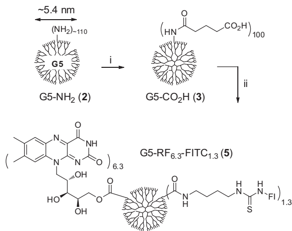
Scheme 1. Synthesis of PAMAM G5-RF-FITC nanoconjugate 5 . Reagents and conditions: (i) glutaric anhydride, Et 3 N, MeOH, rt, 3 days; (ii) riboflavin, FITC-NH(CH 2 ) 4 NH 2 ( 4 ), EDC, DMAP, DMF, rt.
