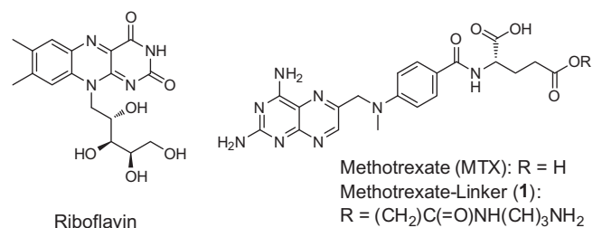
Figure 1. Structure of riboflavin (RF), methotrexate (MTX), and its linker derivative 1.
